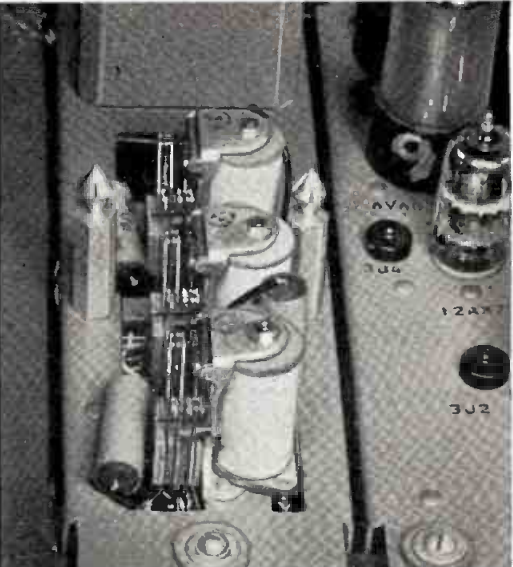
Improved, faster-operating speaker relays eliminate key clicks and audio feedback.
